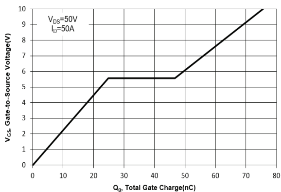
Fig. 11 Gate Charge
