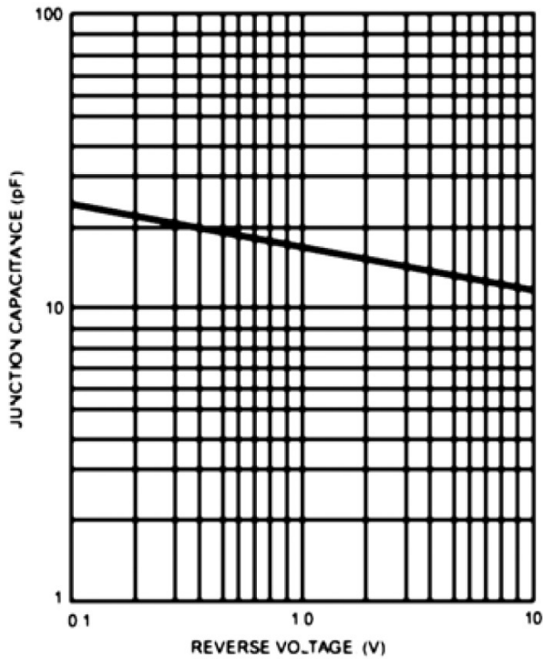
FIG.3- TYPICAL JUNCTION CAPACITANCE
