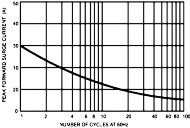
FIG.1- MAXIMUM NON-REPETITIVE FORWARD SURGE CURRENT
