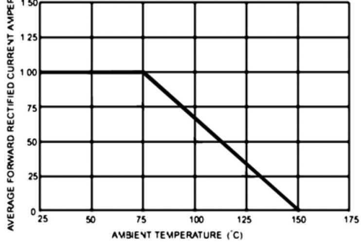
FIG.2- MAXIMUM FORWARD CURRENT DERATING CURVE
