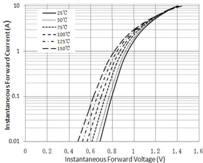
Figure 5. Typical Instantaneous Forward Characteristics
