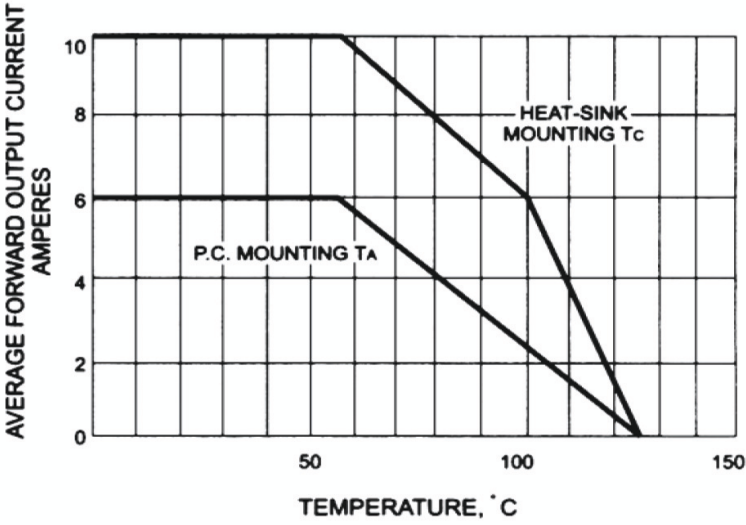
FIG. 2 - DERATING CURVE OUTPUT RECTIFIED CURRENT
