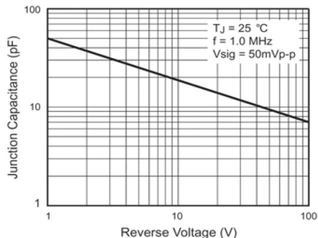
Figure 5. Typical Junction Capacitance Per Leg
