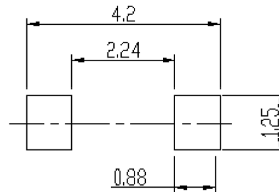
Soldering footprint
