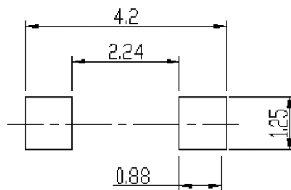
Soldering footprint
