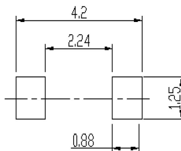
Soldering footprint
