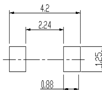
Soldering footprint
