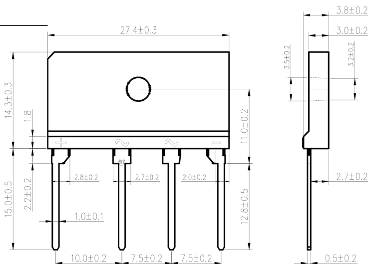
Package Dimensions in mm
