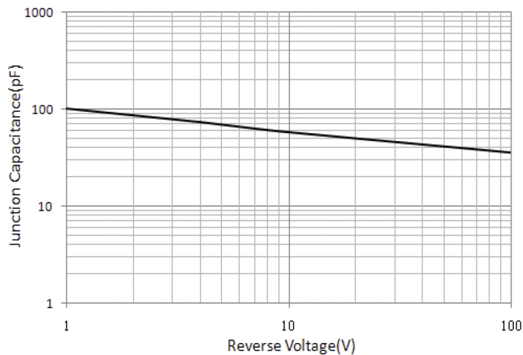
Figure 5. Typical Junction Capacitance Per Leg
