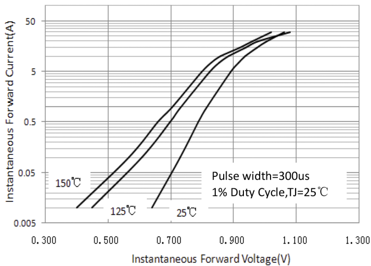
Figure 3. Typical Forward Characteristics Per Leg
