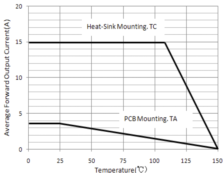
Figure 1. Derating Curve Output Rectified Current
