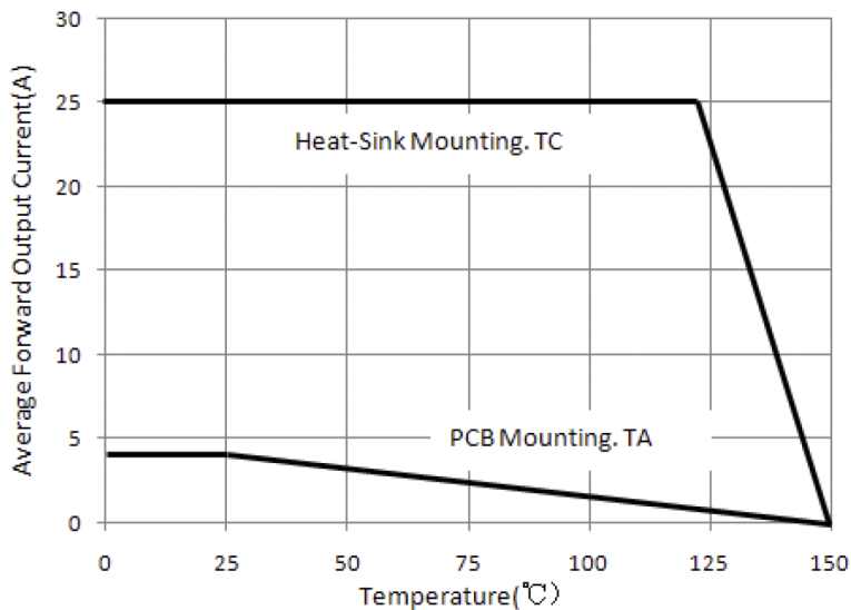
Figure 1. Derating Curve Output Rectified Current
