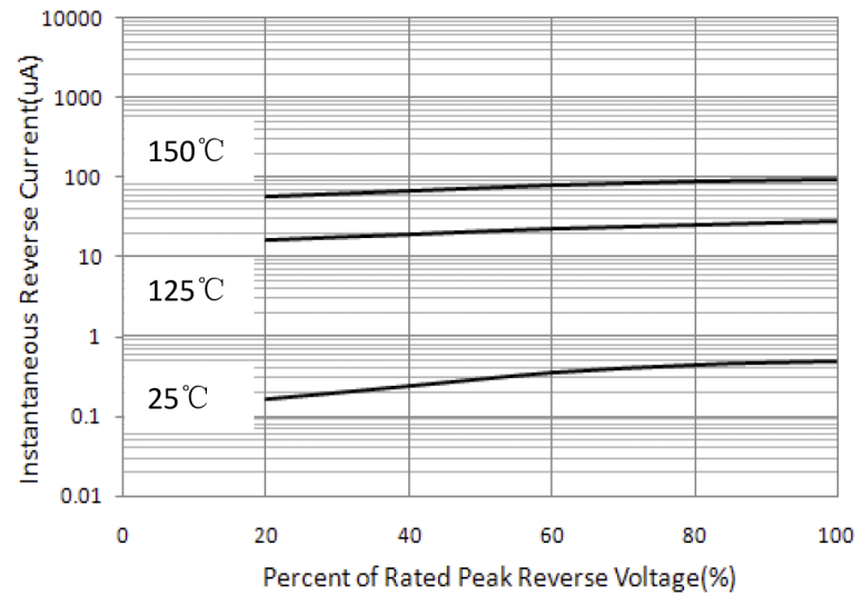
Figure 4. Typical Reverse Characteristics Per Leg
