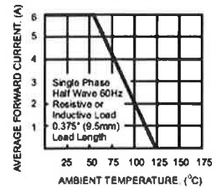
FIG.2- MAXIMUM AVERAGE FORWARD CURRENT DERATING
