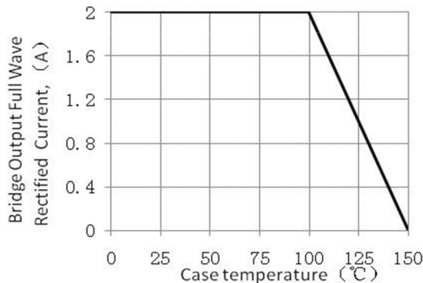
Figure 1. Forward Current Derating
