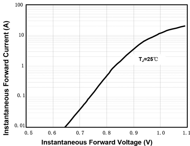
Figure 3. Typical Forward Characteristics Per Diode
