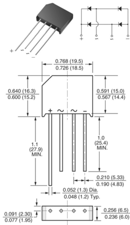
Package outline dimensions in inches (millimeters)
