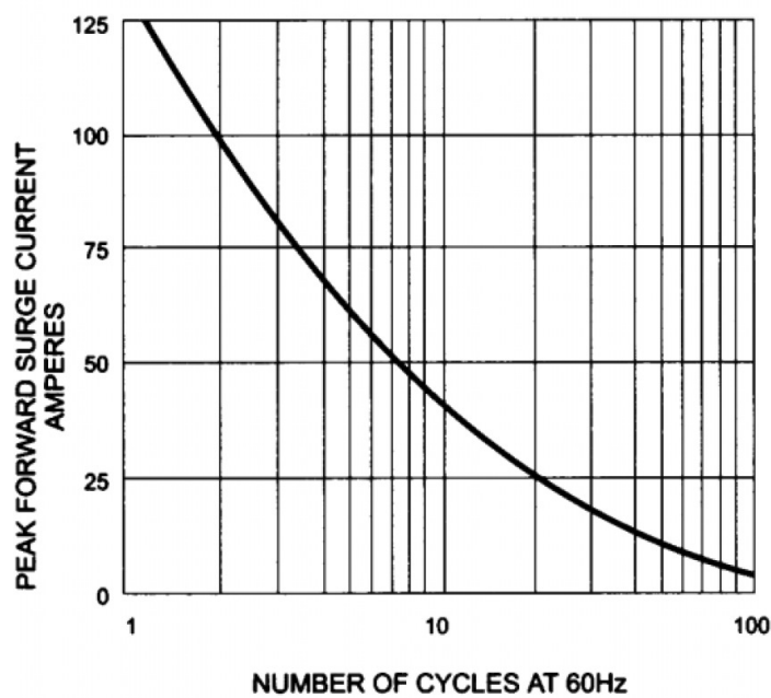
FIG. 1 - MAXIMUM FORWARD SURGE CURRENT
