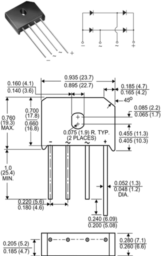
Package outline dimensions in inches (millimeters)
