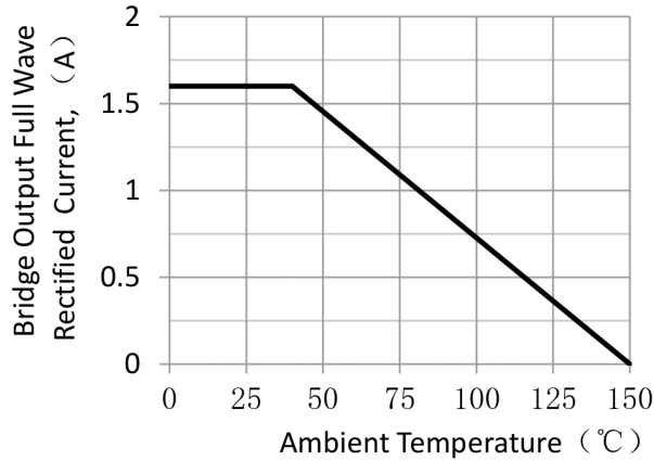
Figure 1. Output Rectifier Current Derating Curve
