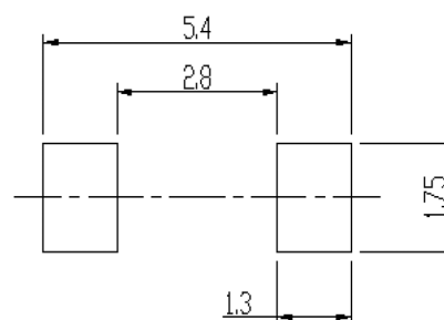
Soldering footprint
