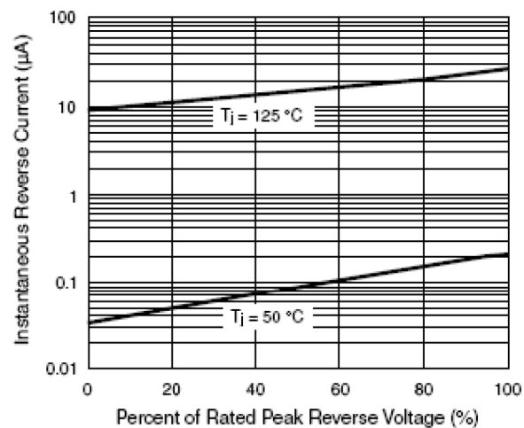
Figure 4. Typical Reverse Leakage Characteristics Per Diode
