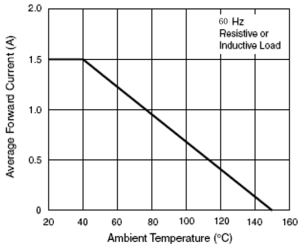
Figure 1. Forward Current Derating Curve Per Diode
