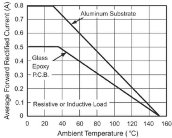
Figure 1. Derating Curve for Output Rectified Current
