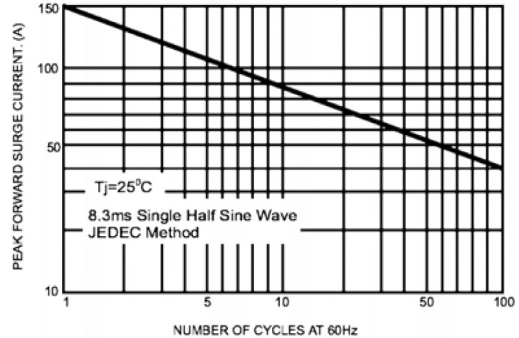
FIG.2- MAXIMUM NON-REPETITIVE PEAK SURGE CURRENT
