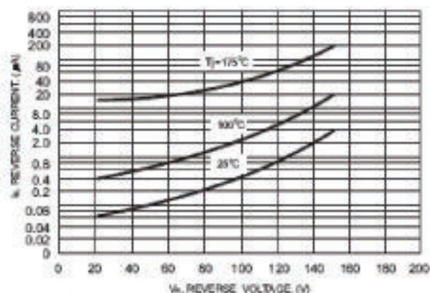
FIG.2- TYPICAL REVERSE CURRENT, PER LEG
