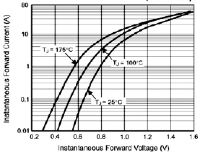
Fig. 3 – Typical Instantaneous Forward Characteristics (MURS120)
