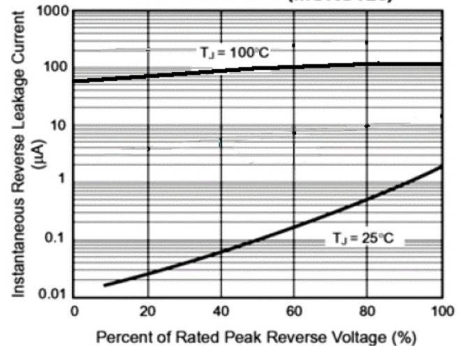
Fig. 4 – Typical Reverse Leakage Characteristics (MURS120)
