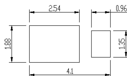
Soldering footprint
