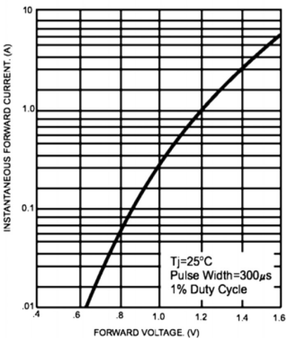
FIG.5- TYPICAL FORWARD CHARACTERISTICS
