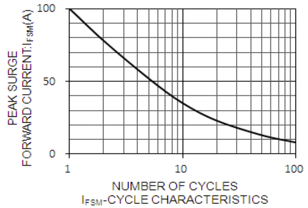
FIG. 2 – MAXIMUM NON-REPETITIVE AVERAGE FORWARD SURGE CURRENT
