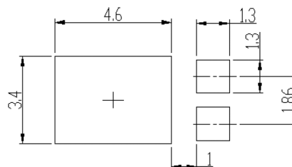
Soldering footprint
