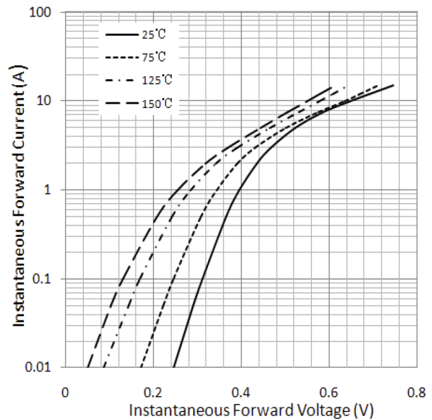
Figure 4. Typical Instantaneous Forward Characteristics
