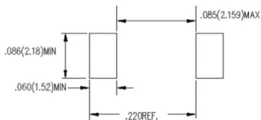
MOUNTING PAD LAYOUT
