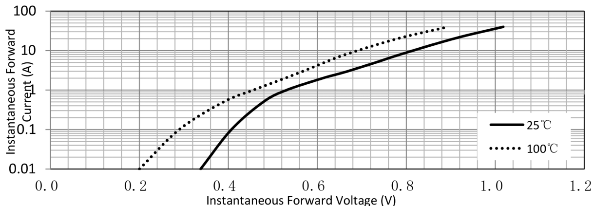
Figure 3. Typical Instantaneous Forward Characteristics
