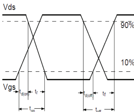
Fig.1-2 Switching Waveform
