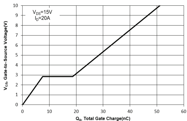
Fig. 11 Gate Charge
