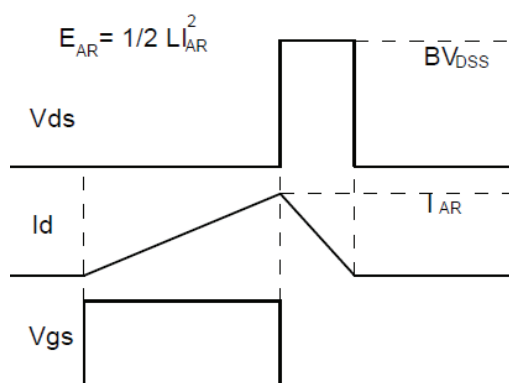
Fig.3-2 Avalanche waveform
