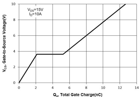
Fig. 11 Gate Charge
