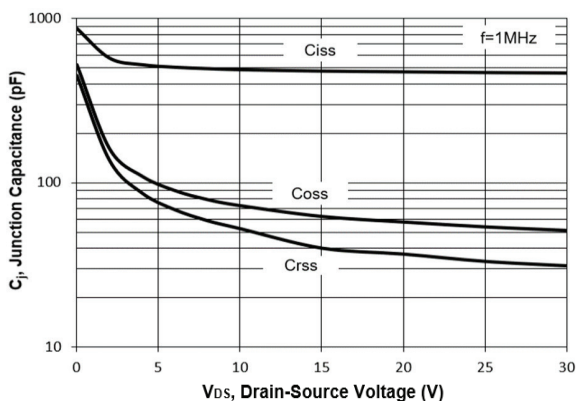
Fig. 7 Typical Junction Capacitance
