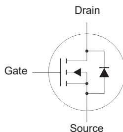
1. Source 2. Source 3. Source 4. Gate 5. Drain 6. Drain 7. Drain 8. Drain DFN3030 Plastic Package
