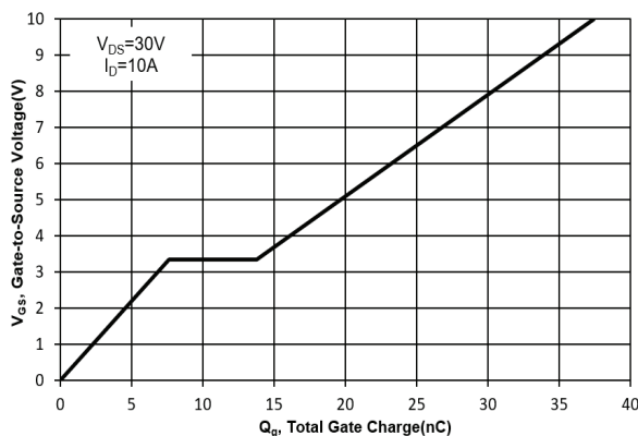
Fig. 11 Gate Charge
