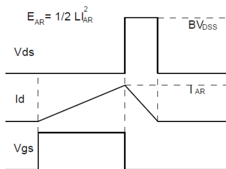
Fig.3-2 Avalanche waveform
