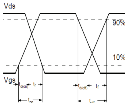
Fig.1-2 Switching Waveform
