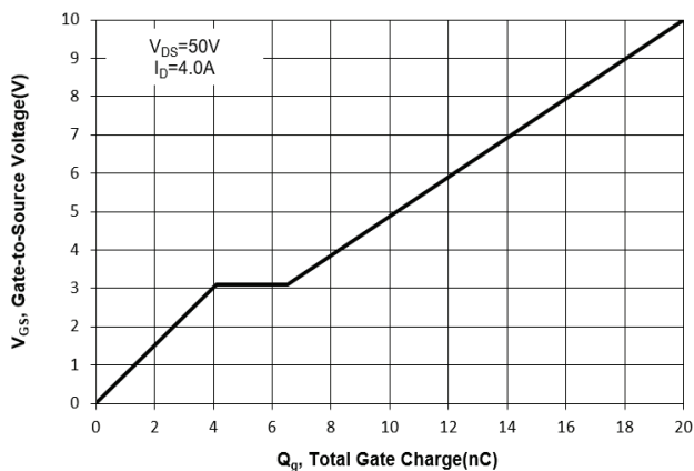
Fig. 11 Gate Charge
