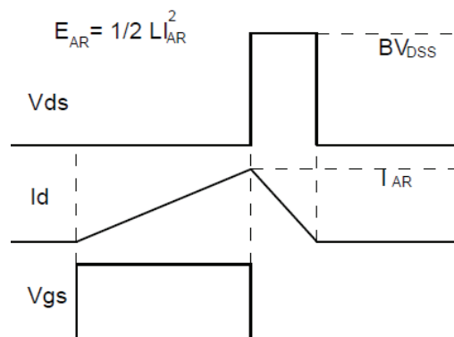
Fig.3-2 Avalanche waveform
