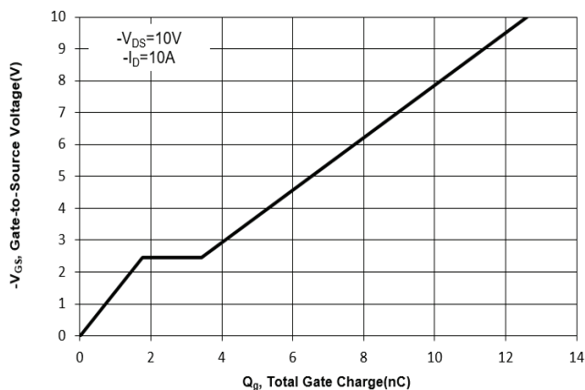
Fig. 11 Gate Charge
