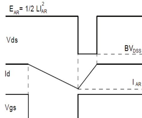
Fig.3-2 Avalanche waveform
