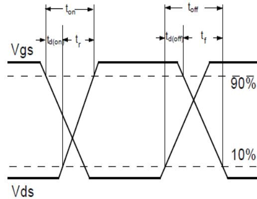
Fig.1-2 Switching Waveform
