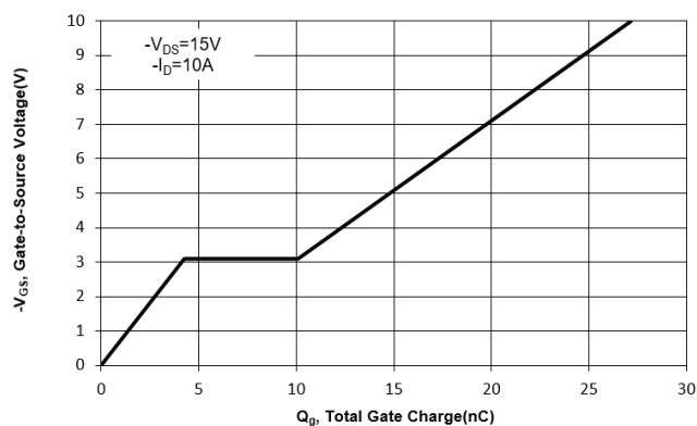
Fig. 11 Gate Charge
