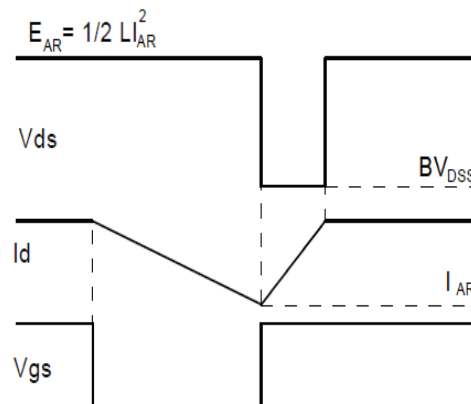
Fig.3-2 Avalanche waveform
