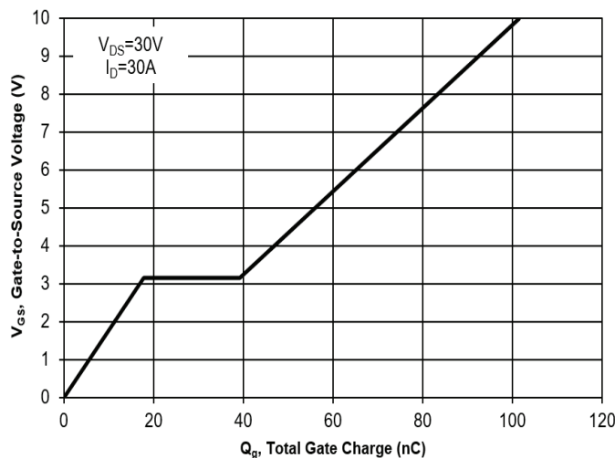
Fig. 11 Gate Charge
