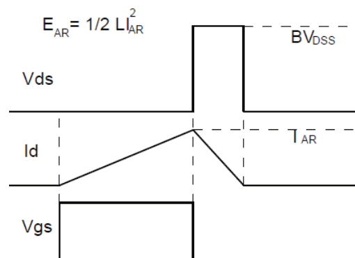
Fig.3-2 Avalanche waveform
