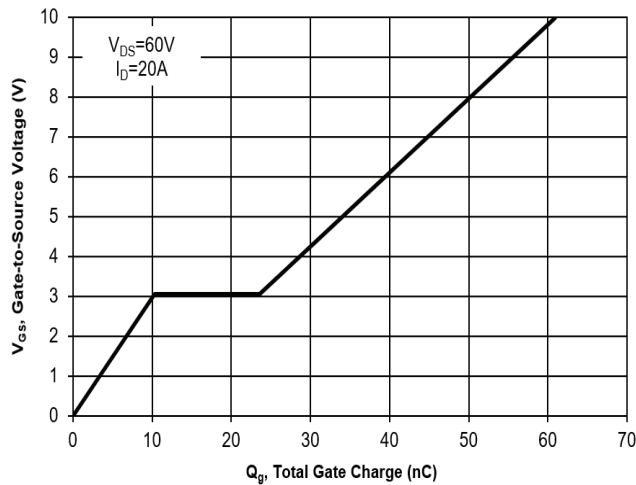
Fig. 11 Gate Charge
