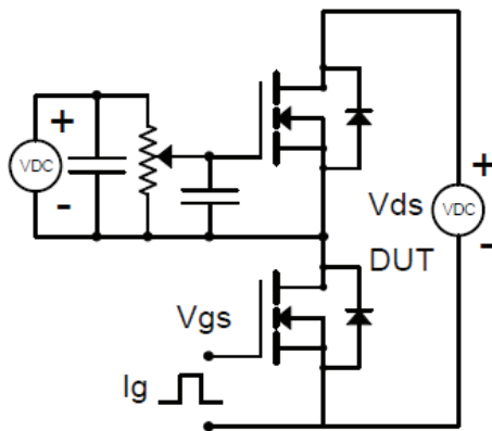
Fig.3-1 Avalanche test circuit
