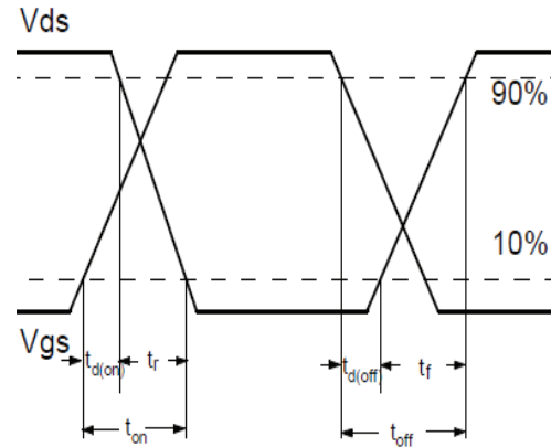
Fig.1-2 Switching Waveform
