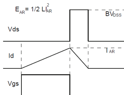
Fig.3-2 Avalanche waveform
