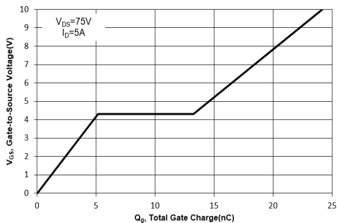
Fig. 11 Gate Charge
