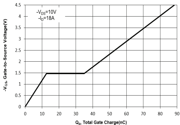
Fig. 11 Gate Charge
