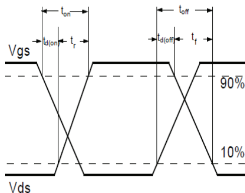
Fig.1-2 Switching Waveform
