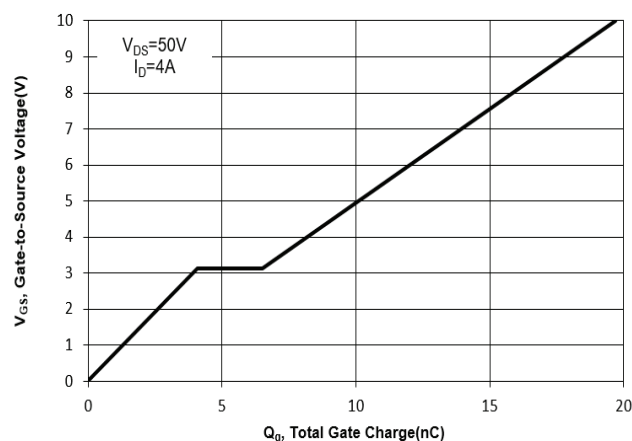
Fig. 11 Gate Charge
