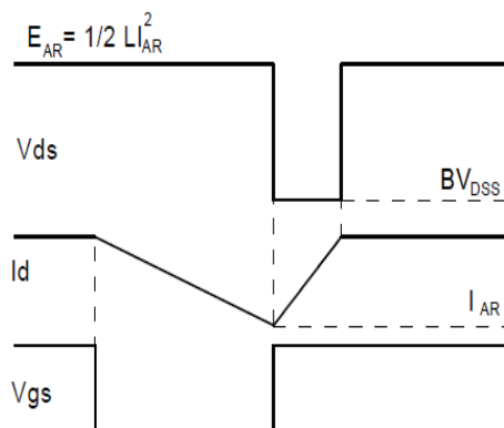
Fig.3-2 Avalanche waveform
