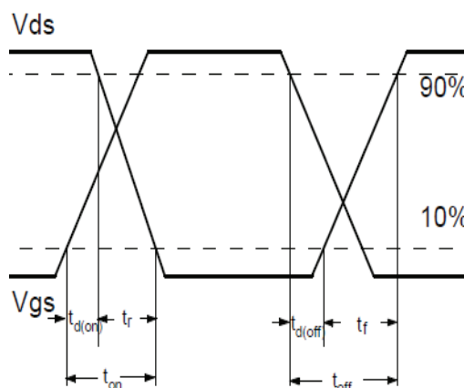
Fig.1-2 Switching Waveform
