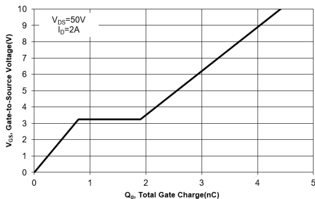
Fig. 11 Gate Charge
