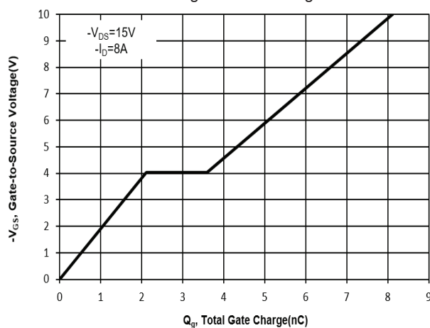
Fig. 11 Gate Charge
